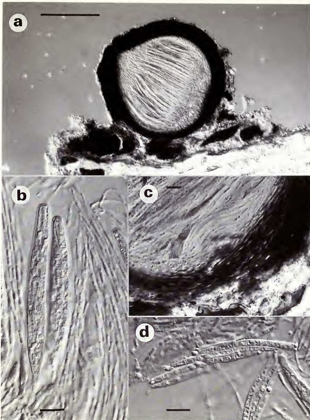
Fig. 47 Cresporhaphis pinicola (G. Samp.) Aguirre (LISU 511—neotype) (a) Vertical section of ascoma, showing involucrellum; scale = 100 \mu m; (b) Asci, ascospores and paraphyses; (c) Detail of exciple: textura angularis to prismatica; (d) Ascospores; scale = 10 \mu m.
